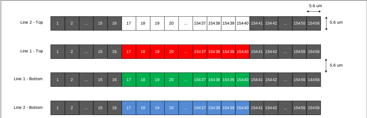
Figure 21: Pixel distribution on 4LS15K RGB + monochrome
