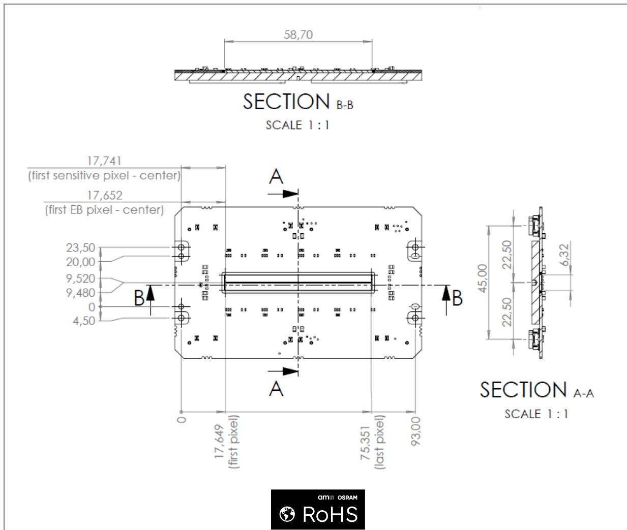
Figure 55: 4LS10K invar package outline drawing – section A-A and section B-B (1)(2)(3)(4)
