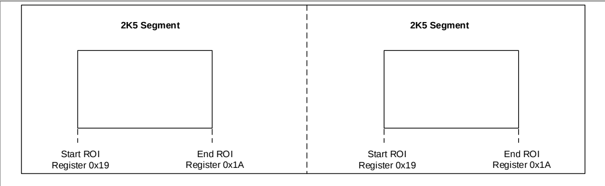
Figure 42: Centered ROI
