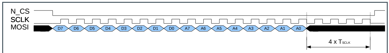
Figure 45: Write cycle over SPI interface
