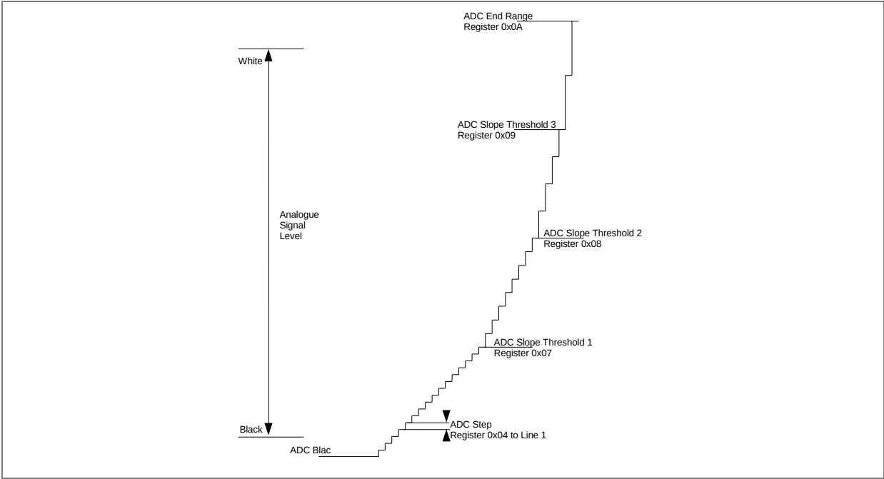
Figure 28: Principle of ADC companding mode
