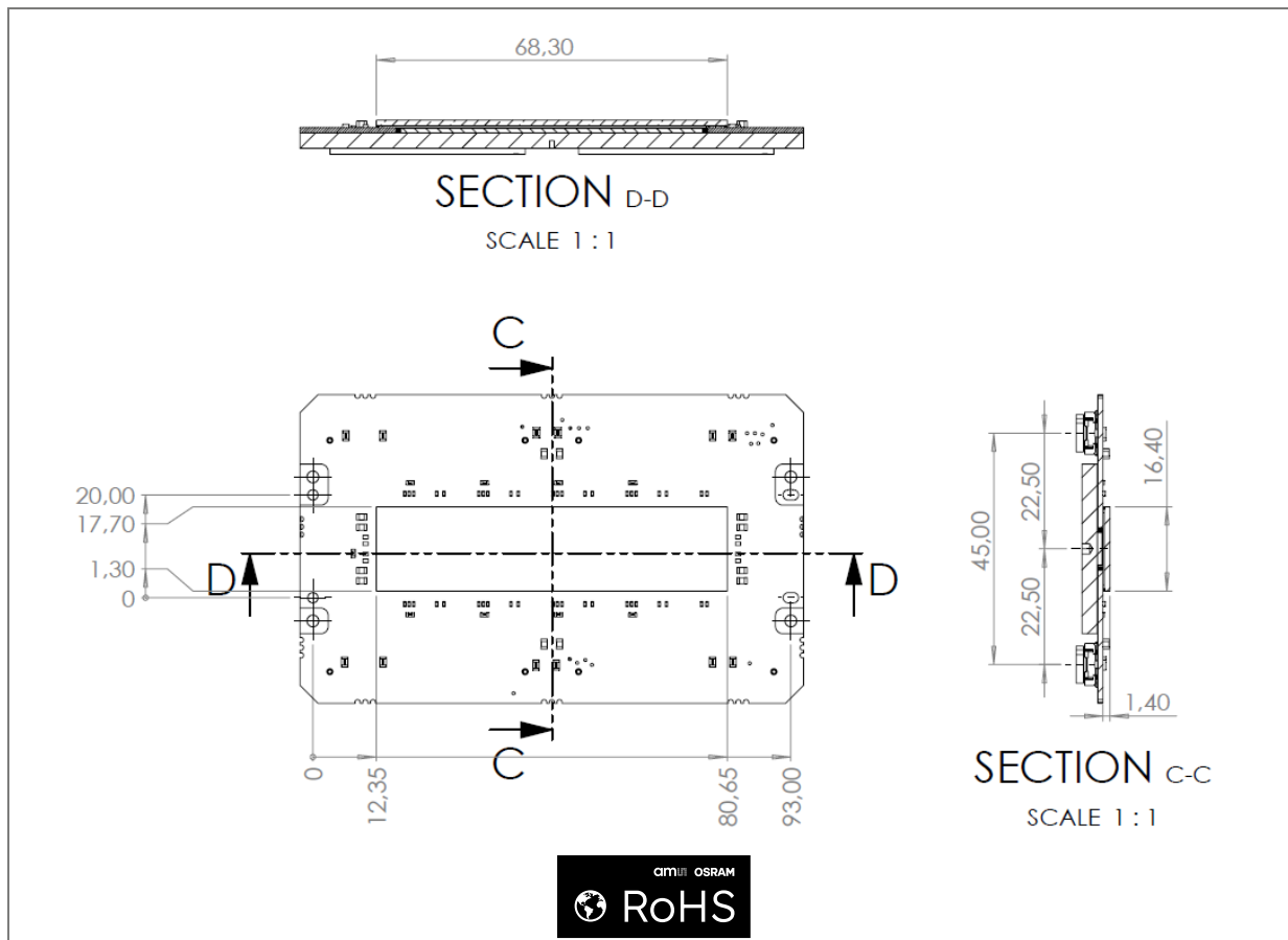
Figure 56: 4LS10K invar package outline drawing – section C-C and section D-D (1)(2)(3)(4)
