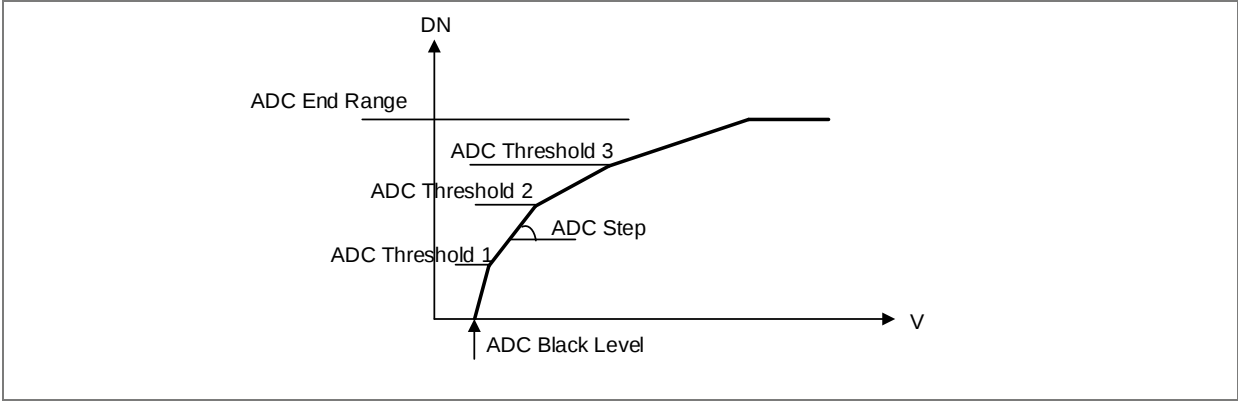
Figure 27: ADC transfer function in companding mode
