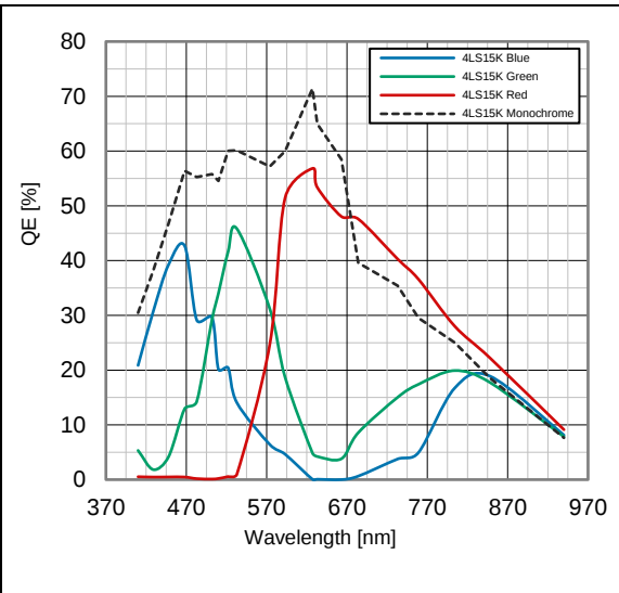
Figure 15: 4LS RGB + monochrome QE
