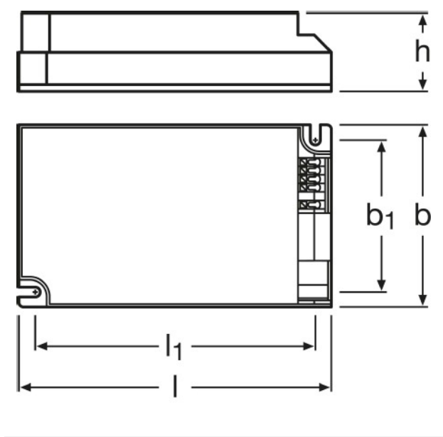
Product line drawing OTp DALI 35/220...240/700 HD
