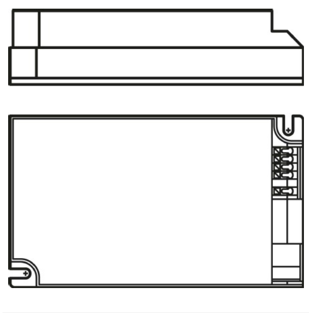
Prod.line drw, front, no dimensions OTp DALI 35/220...240/700 HD
