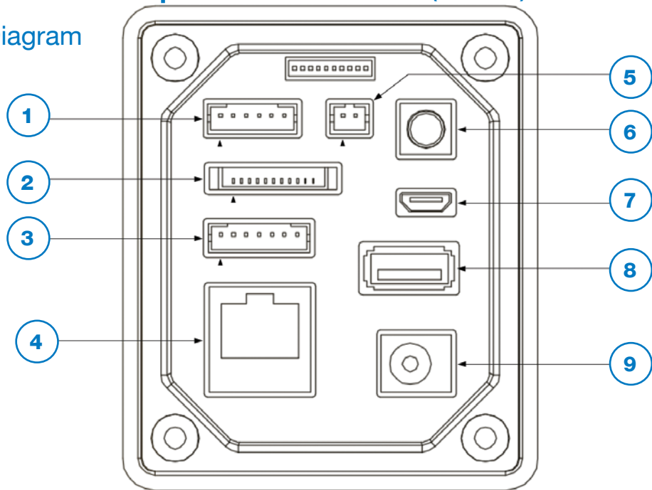
1 6-PIN Open Button, Door Check, Fire Interface
