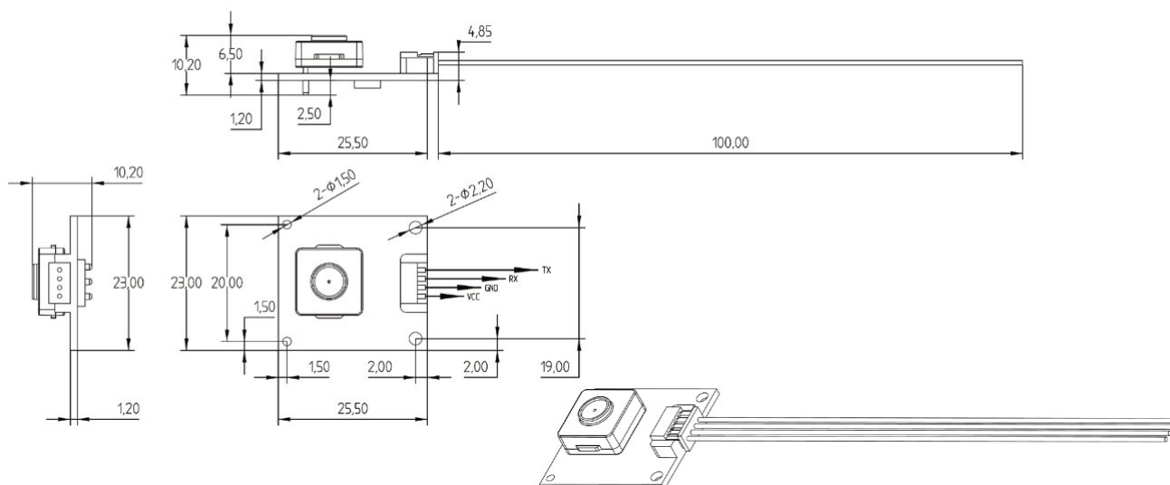
PS1-H2S-100-MOD Dimension diagram (unit: mm)
