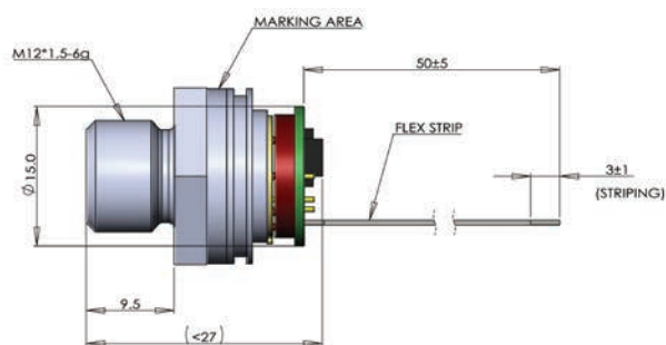
NPI-19M Dimensions (mm)
