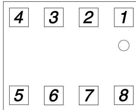
Figure 2 - PKG Diagram
