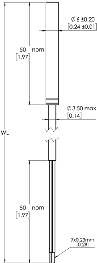
NTC Type JIC - Dimensions
