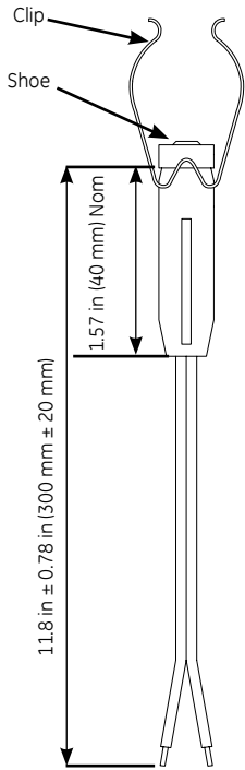
NTC Type JW dimensions
