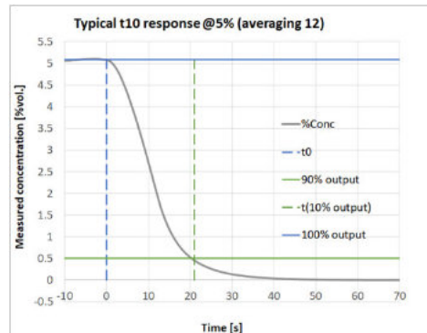
Typical recovery time @5%
