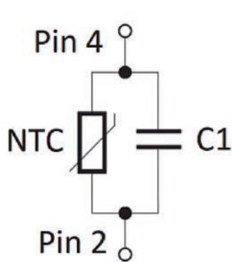
Figure 1: NTC Circuitry
