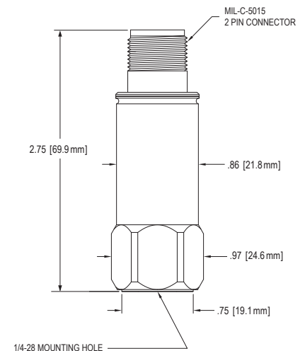
Connections - PCH420V-R6
