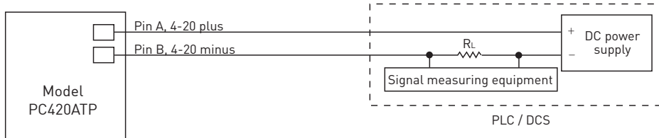
Typical circuit
