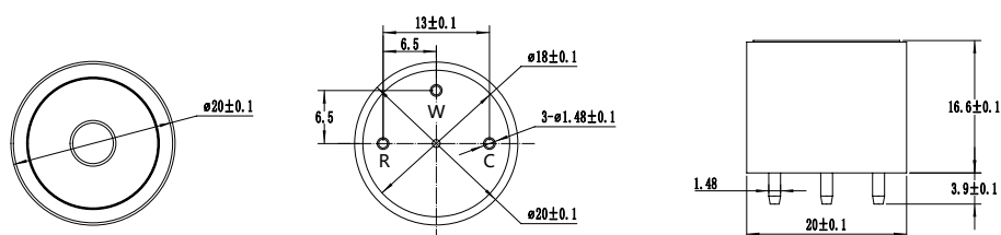
PS4-H2S-5000
