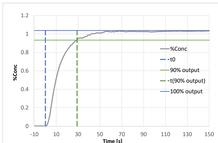
Typical t90 response @1.05% Propane (averaging 20s)
