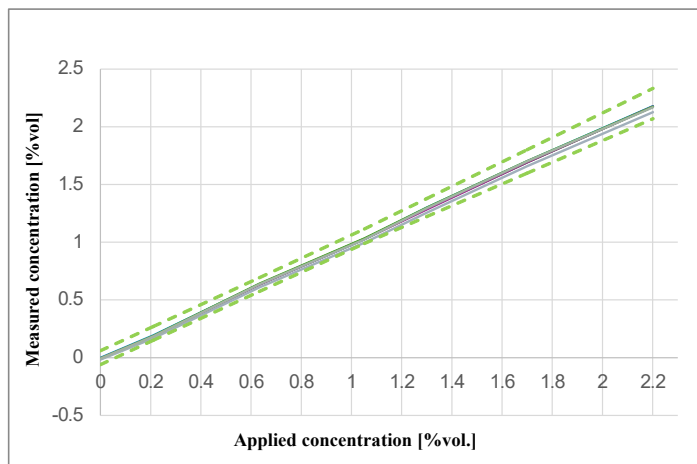
Typical linearity 0-2.1% Propane
