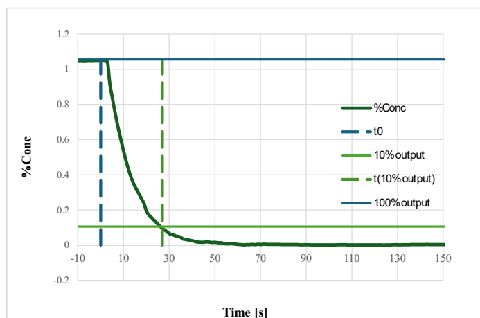
Typical t10 response @1.05% Propane (averaging 20)
