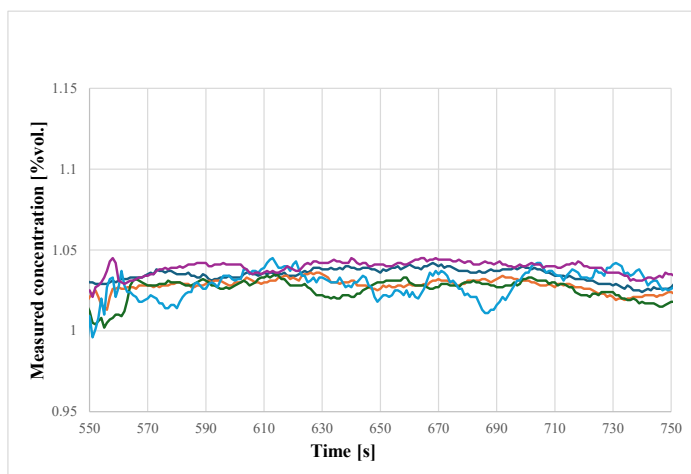
Typical Short Term Stability @1.05% Propane
