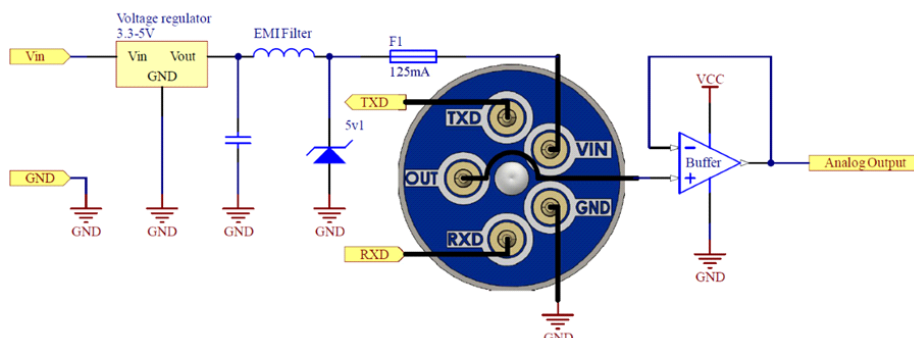
Fig.1 Example schematic for Interfacing Integrated IR (INIR2ia-ME100)
