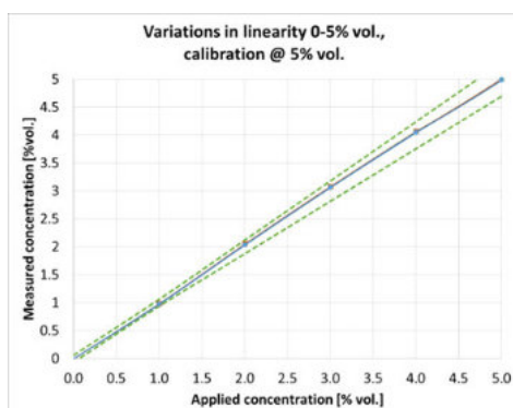
Typical Linearity 0-5%
