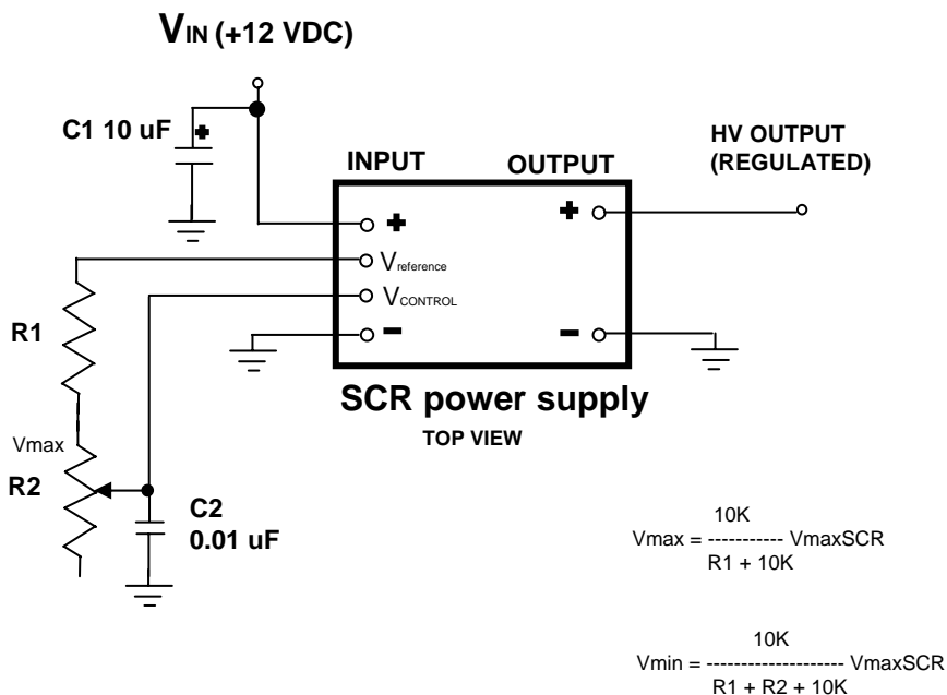
Figure 3: Resistance Programming
