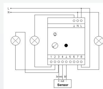
Wiring Example
