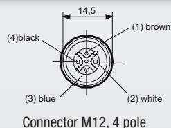
Connector M12, 4 pole
