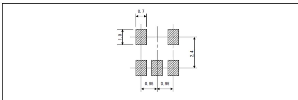
Figure 4-2 Footprint
