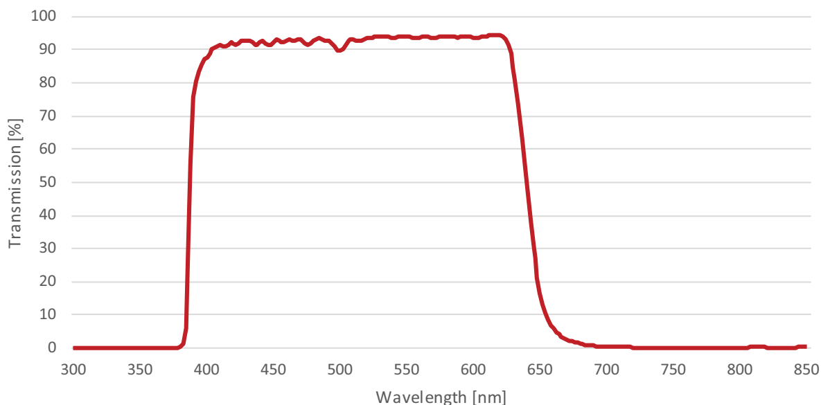
Figure 3: IR cut filter spectral transmission
