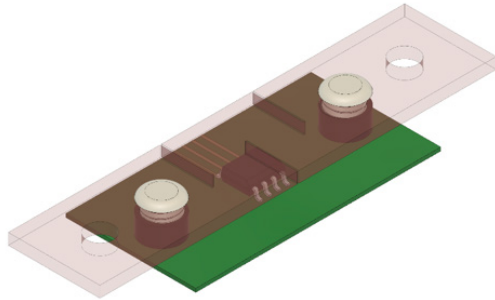
Figure 21: CT453 for Contactless Current Sensing Using Busbar
