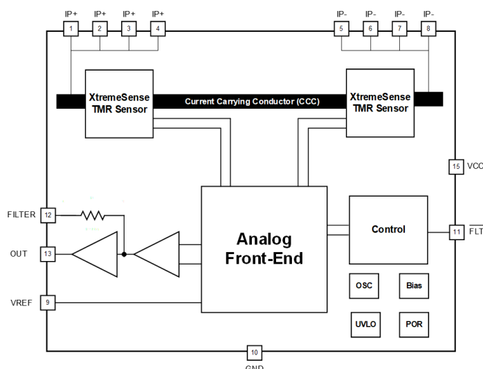
Figure 1: CT431 Functional Block Diagram for 16-lead SOICW Package
