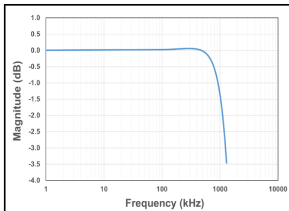
Figure 7: CT416 Bandwidth with C_{FILTER} = 1.0\text{ pF}
