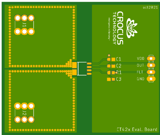
Figure 16: Recommended PCB Layout (Top Layer) for the 20 A to 65 A variants of the CT416
