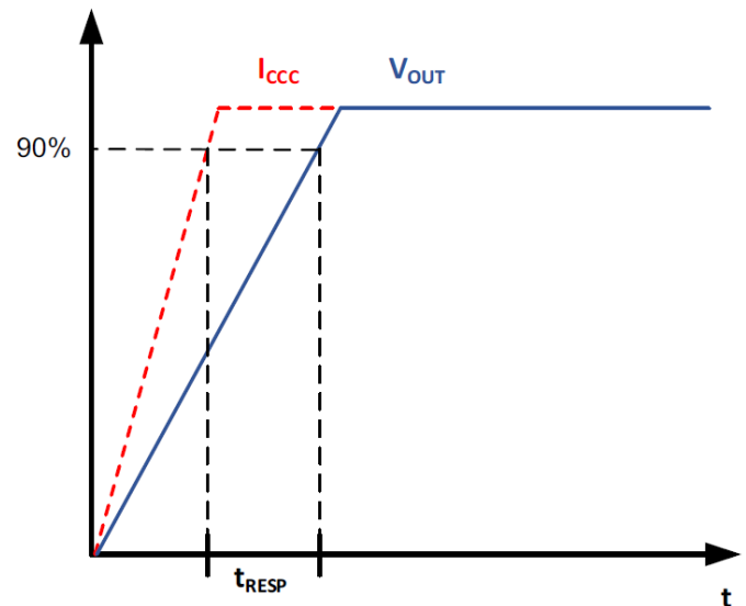
Figure 14: CT416 Response Time Curve
