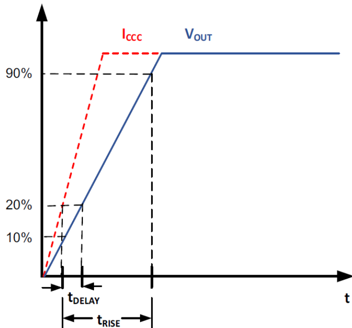
Figure 15: CT416 Propagation Delay and Rise Time Curve
