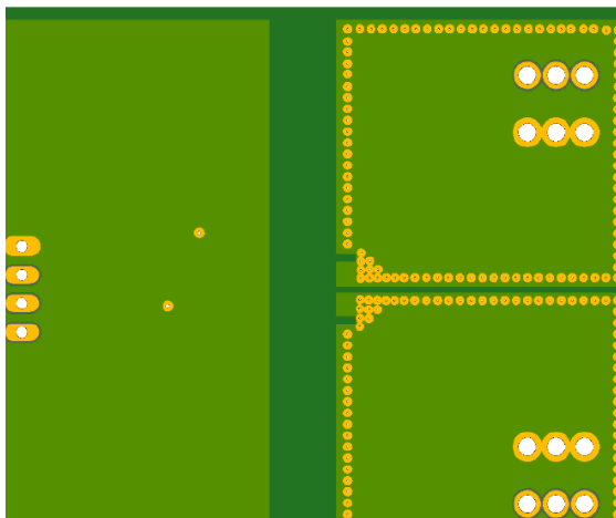
Figure 17: Recommended PCB Layout (Bottom Layer) for the 20 A to 65 A variants of the CT416
