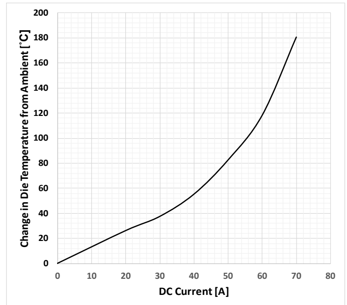
Figure 18: Self Heating in the LA Package Due to Current Flow
