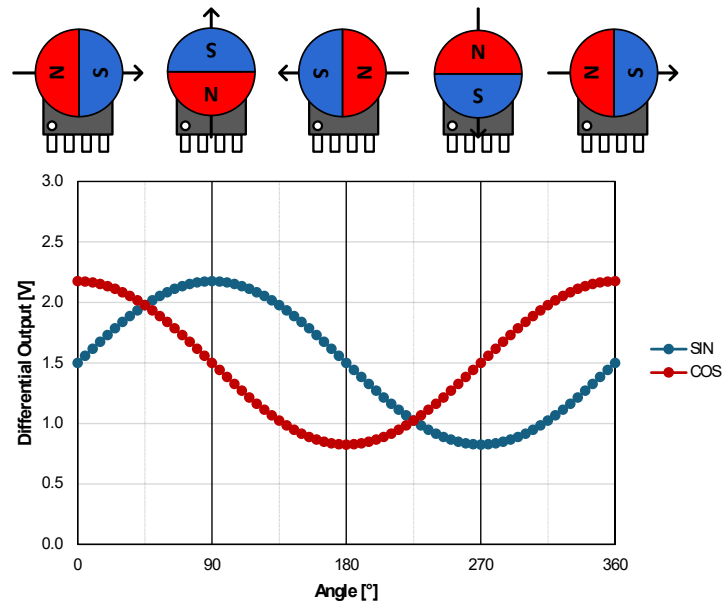
Figure 2: Nominal Differential Output, V_{DD} = 3.0\text{ V}
