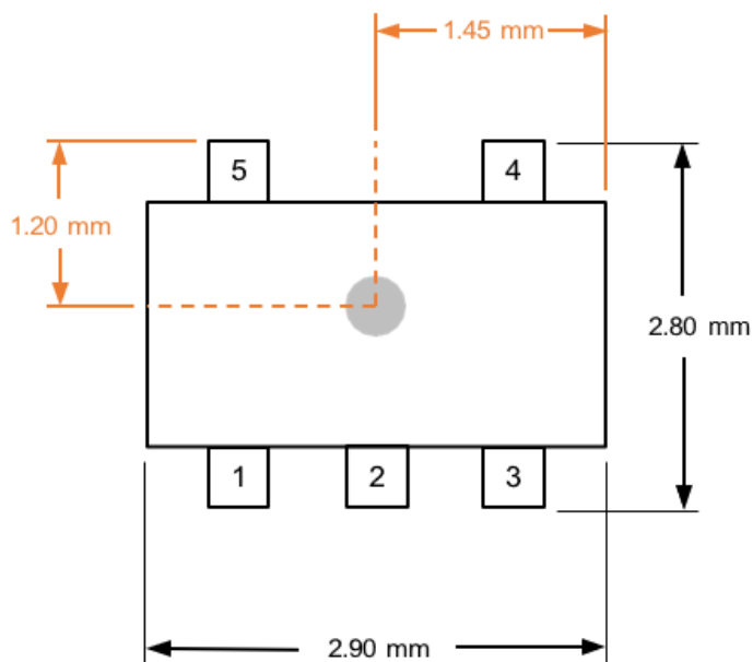
Figure 28: XtremeSense TMR Sensor Location in X and Y Dimensions for CT220 in SOT23-5 Package
