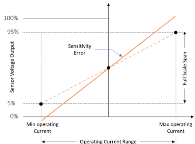
Figure 21: Exaggerated Gain Error
