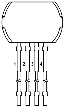
Pinout Diagram
