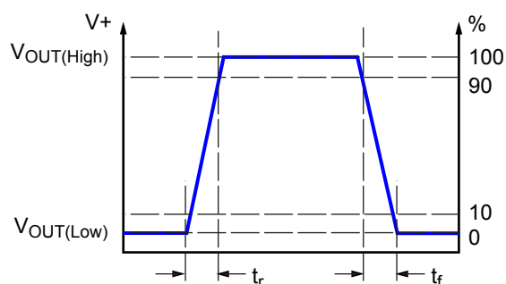
Figure 2. Output Rise Time and Output Fall Time
