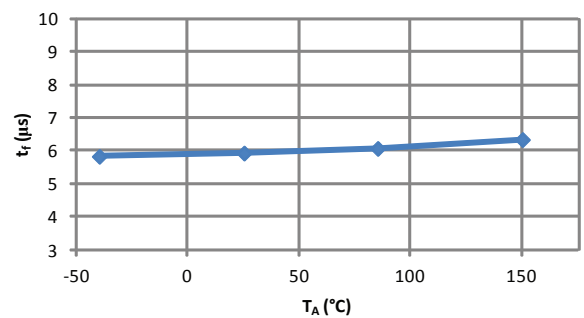
Output Fall Time versus Ambient Temperature
