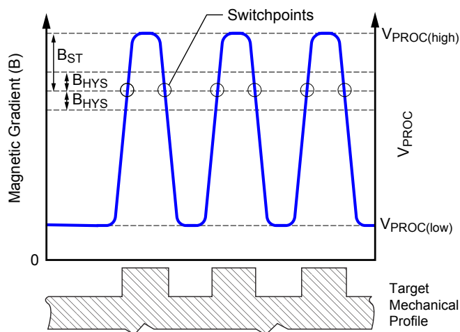
Figure 4. Running Mode Switch Point and Internal Hysteresis
