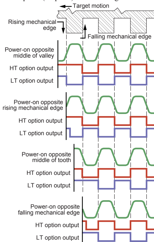
Figure 6. Start-up behavior (when connected as shown in figure 1)
