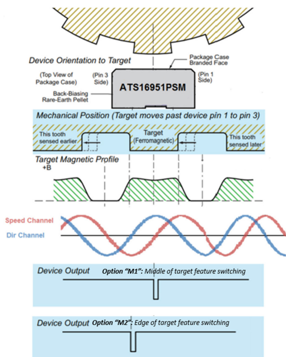
Figure 8: Magnetic Profile
