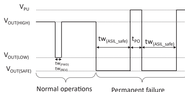
Figure 11: ASIL Output Behavior (ASIL Option -A)
