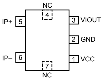
Pinout Diagram
