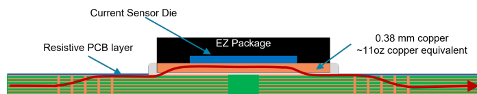
Figure 13: No In-Pad Vias
