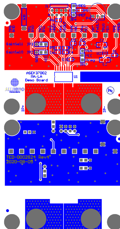
Figure 21: Top and Bottom Layers for ASEP37002 Evaluation Board
