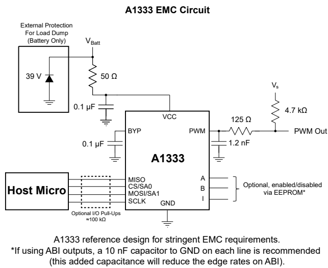
Figure 56: A1333 PWM/ABI, SPI, and EMC Application Circuits
