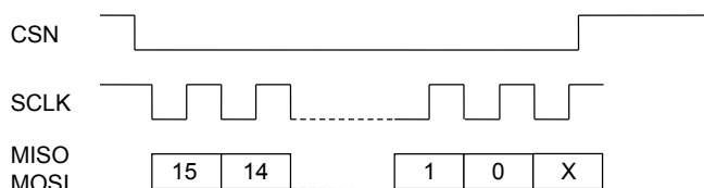
Figure 40: 16-Bit SPI Transaction
