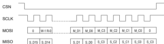
Figure 43: 21-Bit SPI Transaction
