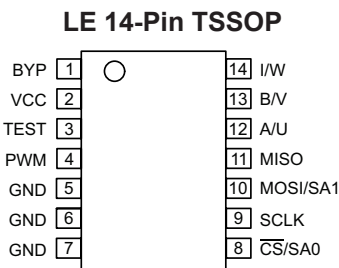
Pinout Diagram
