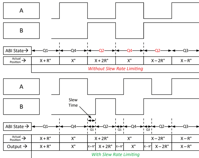
Figure 30: Slew-Rate Limiting
