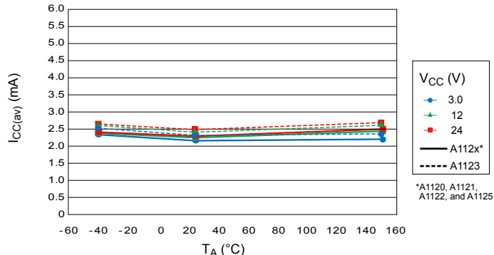
Average Supply Current (Off) versus Ambient Temperature
