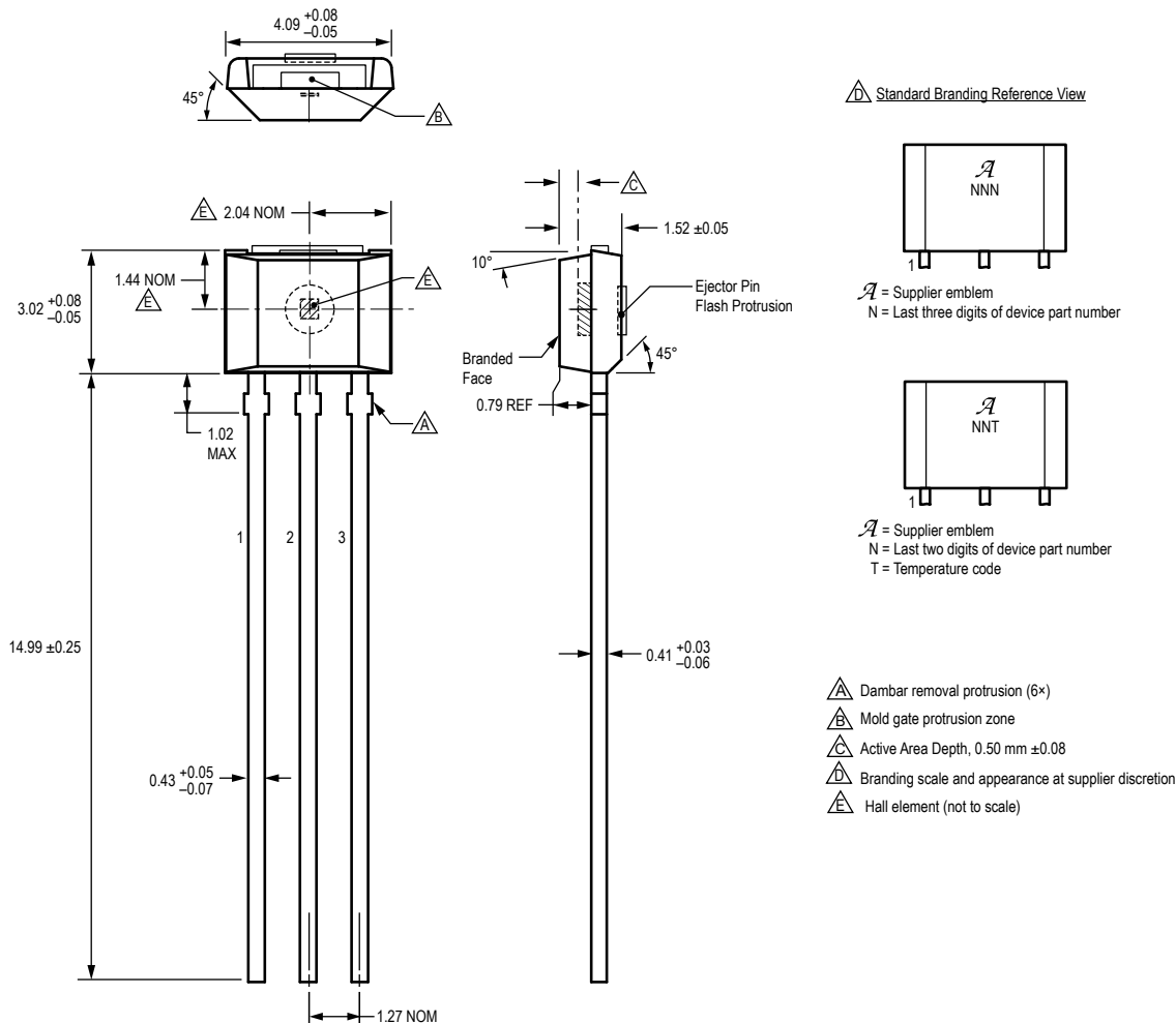
Figure 4: Package UA, 3-Pin SIP, Matrix Style
