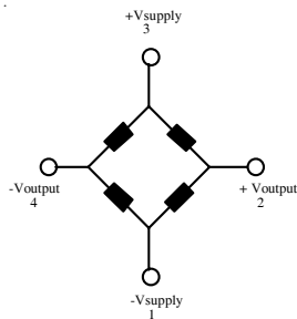
Equivalent Circuit
