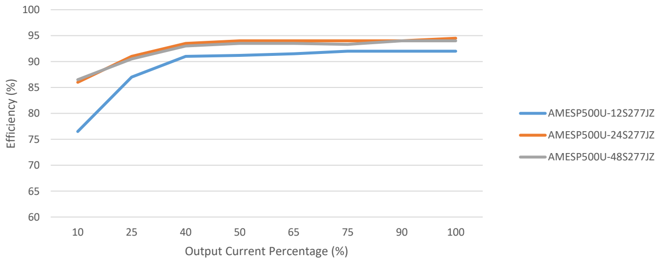
Efficiency vs Output Load (Vin=230VAC)
