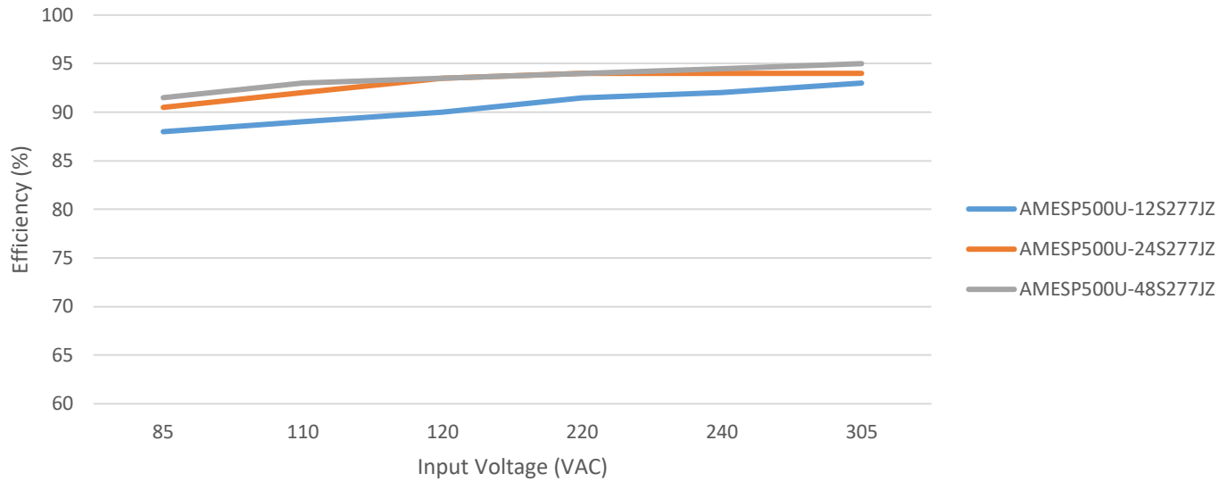
Efficiency vs Input Voltage (Full Load)
