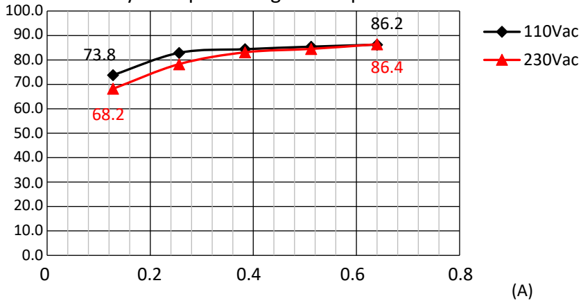
(%) Efficiency Vs. Input Voltage & Output Current
