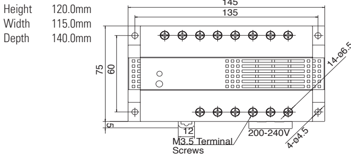
PS5R-E (100W)
