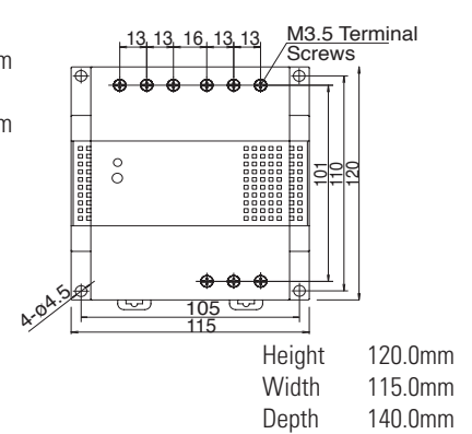
PS5R-F (120W)
