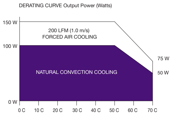
Figure 1: Derating Curve
