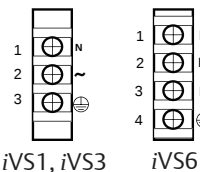
Figure 1. AC Input
