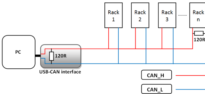
Figure 3-8 Terminating resistors are required for CAN interface
