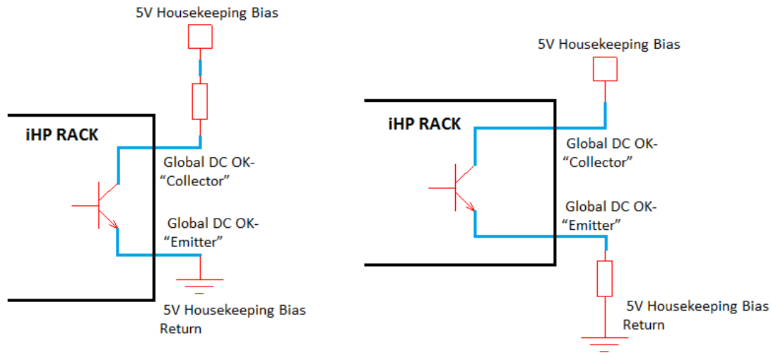
Figure 4-13 Possible circuit configuration for DCOK functionality
