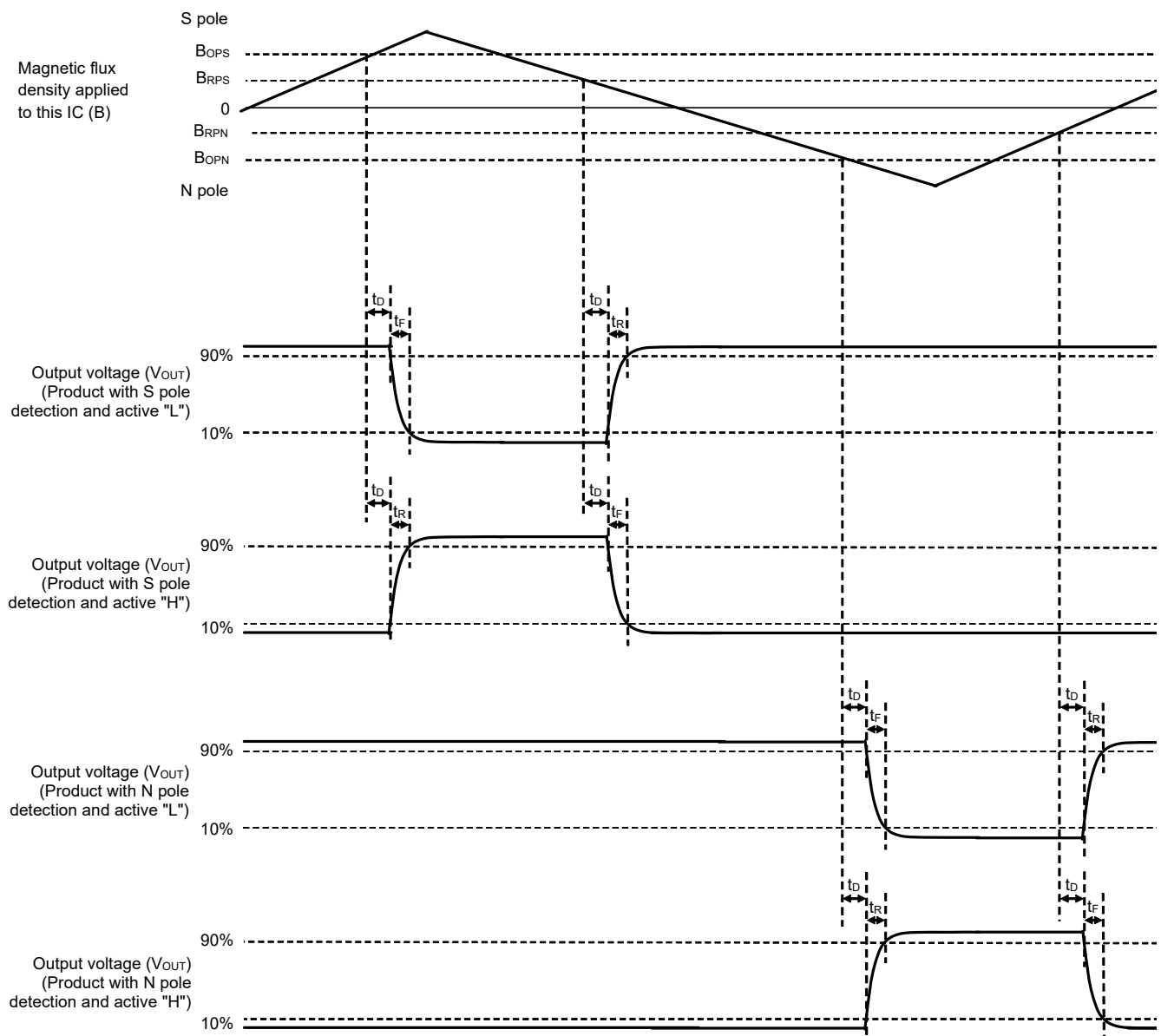
Figure 5 Operation Timing
