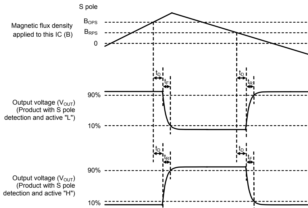
Figure 4 Operation Timing
