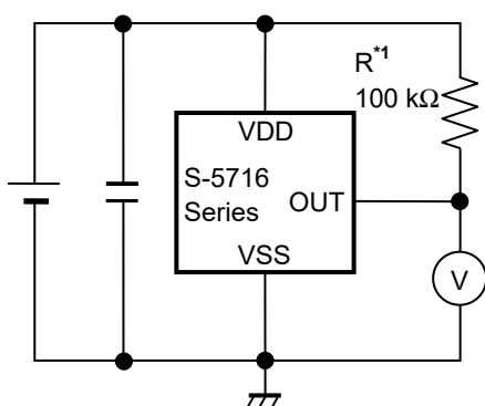
Figure 9 Test Circuit 5
