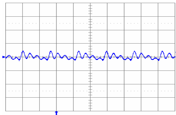
Fig. 1.0V.5: Output voltage ripple (20 mV/div.) at full rated load current into a resistive load with external capacitance 100 \mu F ceramic + 1 \mu F ceramic and V_{in} = 12 V for V_{out} = 1.0 V. Time scale: 2 \mu s/div.
