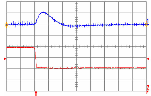
Fig. 0.7525V.7: Output voltage response for V_{out} = 0.7525 V to negative load current step change from 20 A to 10 A with slew rate of -5 A/ \mu s at V_{in} = 12 V. Top trace: output voltage (200 mV/div.); Bottom trace: load current (5 A/div.). C_o = 100 \mu F ceramic. Time scale: 20 \mu s/div.
