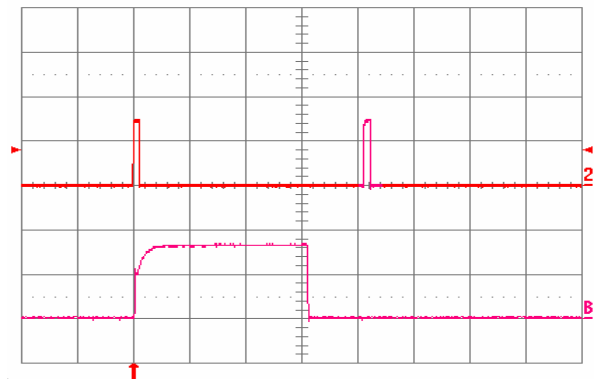
Fig. 16: Load current (top trace, 20 A/div., 50 ms/div.) into a 10 m \Omega short circuit during restart, at V_{in} = 48V . Bottom trace (10 A/div., 2 ms/div.) is an expansion of the on-time portion of the top trace.
