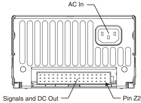
Figure 2. NP1200 Connectors
