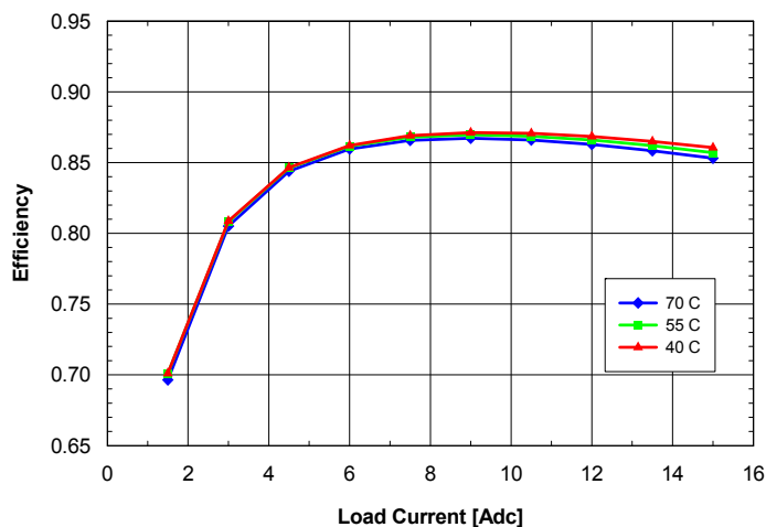
Fig. 2.5V.6: Efficiency vs. load current and ambient temperature for ASQ24T/S15025 converter mounted vertically with V_{in} = 24\text{V} and air flowing from pin 3 to pin 1 at a rate of 200 LFM (1.0 m/s).
