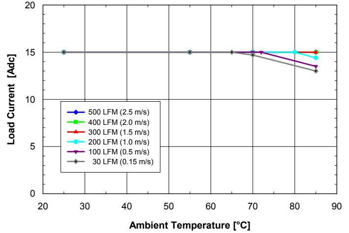
Fig. 2.0V.2: Available load current vs. ambient air temperature and airflow rates for ASQ24T15020 converter with B height pins mounted horizontally with V_{in} = 24V , air flowing from pin 3 to pin 1 and maximum FET temperature \leq 120^{\circ}C .
