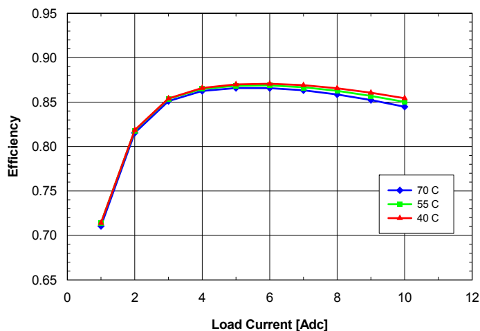
Fig. 5.0V.6: Efficiency vs. load current and ambient temperature for ASQ24T/S10050 converter mounted vertically with V_{in} = 24\text{V} and air flowing from pin 3 to pin 1 at a rate of 200 LFM (1.0 m/s).
