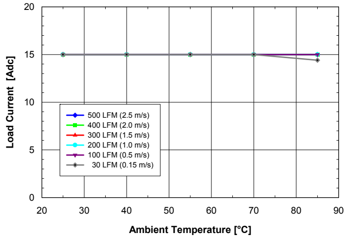
Fig. 1.8V.4: Available load current vs. ambient temperature and airflow rates for ASQ24S15018 converter mounted horizontally with V_{in} = 24V , air flowing from pin 3 to pin 1 and maximum FET temperature \leq 120^{\circ}C .
