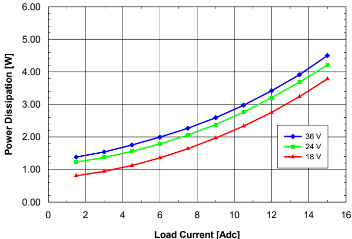
Fig. 1.2V.7: Power dissipation vs. load current and input voltage for ASQ24T/S15012 converter mounted vertically with air flowing from pin 3 to pin 1 at a rate of 300 LFM (1.5 m/s) and T_a = 25^\circ\text{C} .
