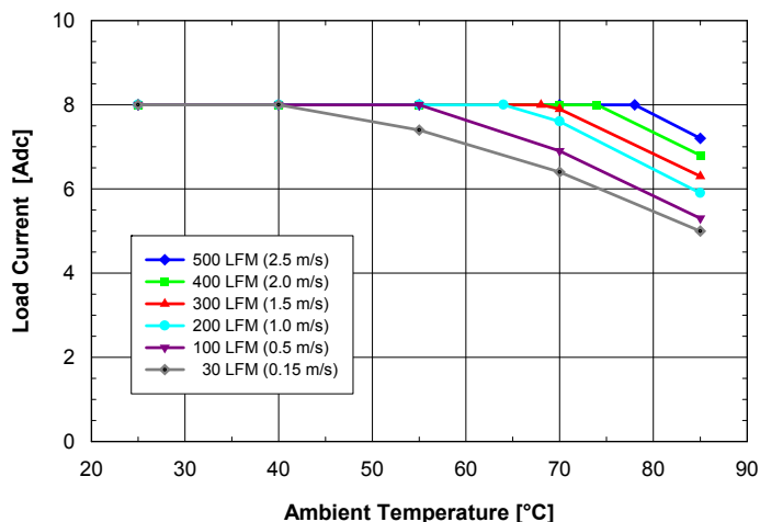
Fig. 6.0V.1: Available load current vs. ambient air temperature and airflow rates for ASQ24T08060 converter with B height pins mounted vertically with V_{in} = 24V , air flowing from pin 3 to pin 1 and maximum FET temperature \leq 120^{\circ}C .
