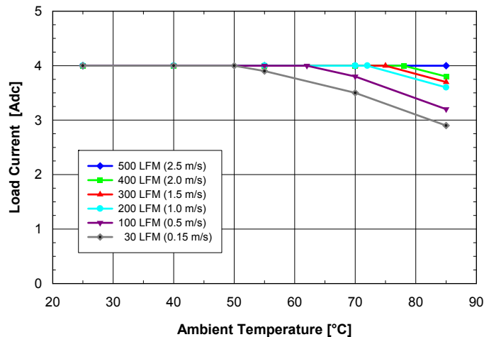
Fig. 12V.4: Available load current vs. ambient temperature and airflow rates for ASQ24S04120 converter mounted horizontally with V_{in} = 24V , air flowing from pin 3 to pin 1 and maximum FET temperature \leq 120^{\circ}C .
