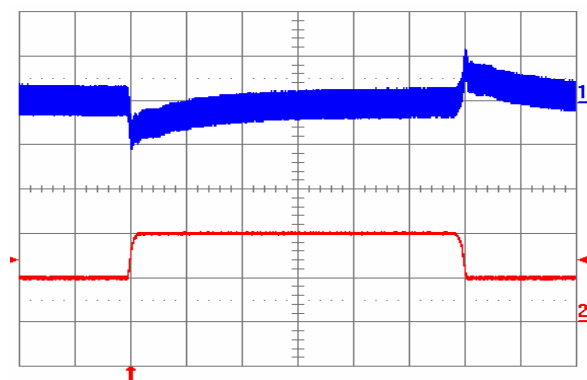
Fig. 6.0V.11: Output voltage response to load current step-change (2A – 4A – 2A) at V_{in} = 24V . Top trace: output voltage (100mV/div.). Bottom trace: load current (2A/div.). Current slew rate: 0.1 A/µs. C_o = 1 \mu F ceramic. Time scale: 0.2 ms/div.
