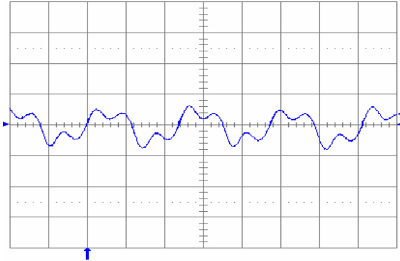
Fig. 2.5V.13: Output voltage ripple (20 mV/div.) at full rated load current into a resistive load with C_o = 10 \mu\text{F} tantalum + 1\mu\text{F} ceramic and V_{in} = 24\text{V} . Time scale: 1 \mu\text{s}/\text{div} .
