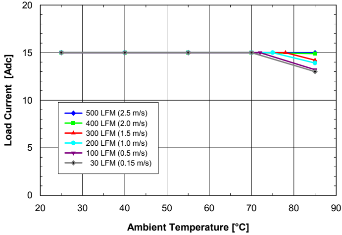
Fig. 2.0V.1: Available load current vs. ambient air temperature and airflow rates for ASQ24T15020 converter with B height pins mounted vertically with V_{in} = 24V , air flowing from pin 3 to pin 1 and maximum FET temperature \leq 120^{\circ}C .
