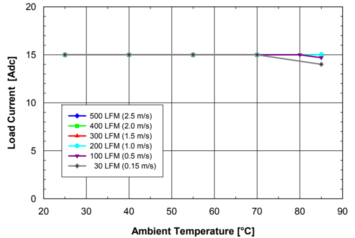
Fig. 2.0V.4: Available load current vs. ambient temperature and airflow rates for ASQ24S15020 converter mounted horizontally with V_{in} = 24V , air flowing from pin 3 to pin 1 and maximum FET temperature \leq 120^{\circ}C .
