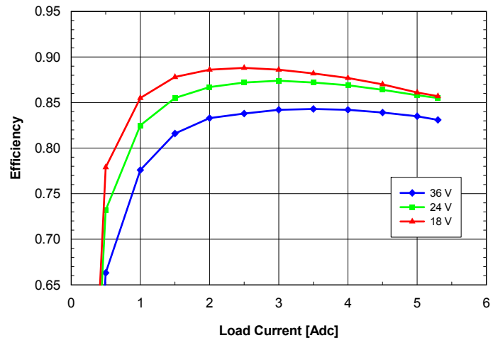
Fig. 8.0V.2: Efficiency vs. load current and input voltage for ASQ24T/S05080 converter mounted vertically with air flowing from pin 3 to pin 1 at a rate of 300 LFM (1.5 m/s) and T_a = 25^{\circ}\text{C} .
