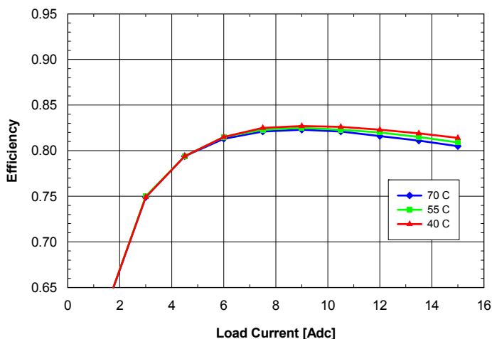
Fig. 1.2V.6: Efficiency vs. load current and ambient temperature for ASQ24T/S15012 converter mounted vertically with V_{in} = 24\text{V} and air flowing from pin 3 to pin 1 at a rate of 200 LFM (1.0 m/s).
