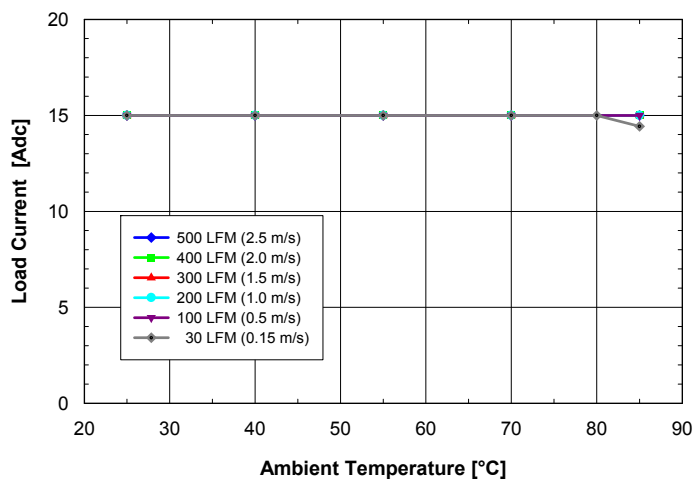
Fig. 1.8V.2: Available load current vs. ambient air temperature and airflow rates for ASQ24T15018 converter with B height pins mounted horizontally with V_{in} = 24V , air flowing from pin 3 to pin 1 and maximum FET temperature \leq 120^{\circ}C .
