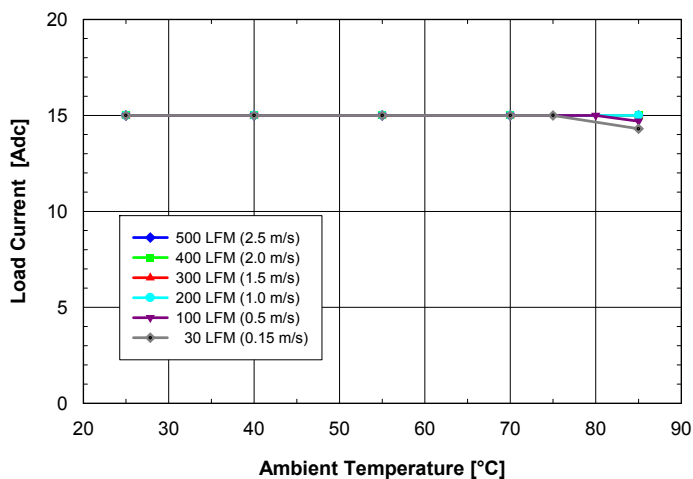
Fig. 1.8V.1: Available load current vs. ambient air temperature and airflow rates for ASQ24T15018 converter with B height pins mounted vertically with V_{in} = 24V , air flowing from pin 3 to pin 1 and maximum FET temperature \leq 120^{\circ}C .
