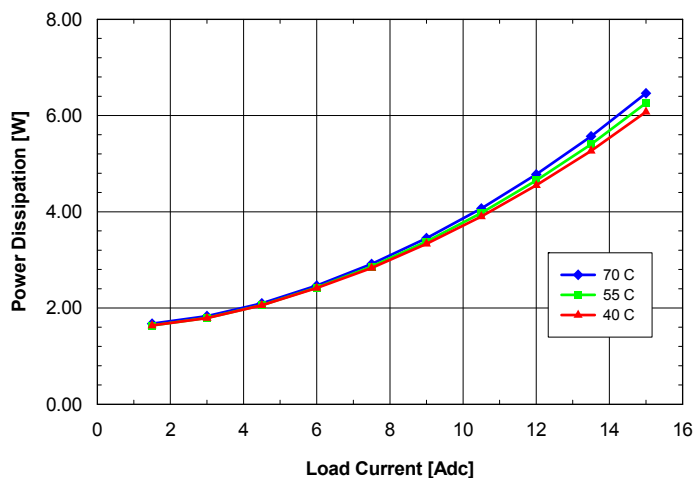
Fig. 2.5V.8: Power dissipation vs. load current and ambient temperature for ASQ24T/S15025 converter mounted vertically with V_{in} = 24\text{V} and air flowing from pin 3 to pin 1 at a rate of 200 LFM (1.0 m/s).
