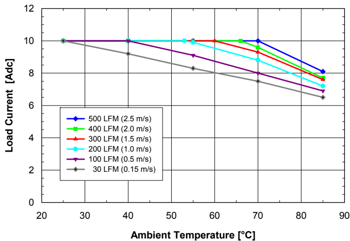
Fig. 5.0V.4: Available load current vs. ambient temperature and airflow rates for ASQ24S10050 converter mounted horizontally with V_{in} = 24V , air flowing from pin 3 to pin 1 and maximum FET temperature \leq 120^{\circ}C .
