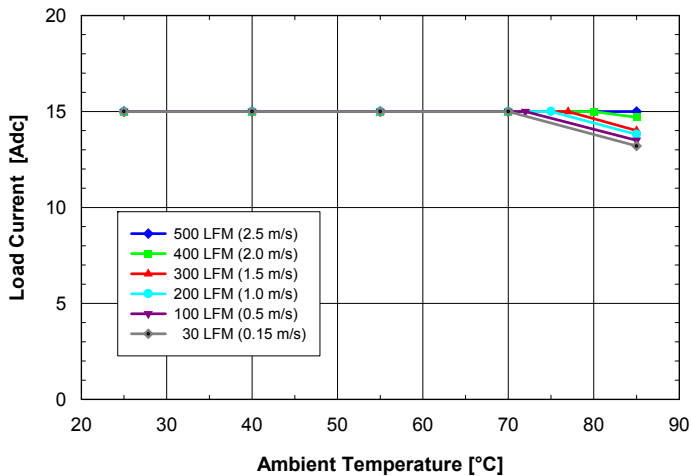
Fig. 2.0V.3: Available load current vs. ambient temperature and airflow rates for ASQ24S15020 converter mounted vertically with V_{in} = 24V , air flowing from pin 3 to pin 1 and maximum FET temperature \leq 120^{\circ}C .
