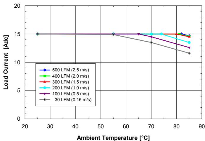
Fig. 2.5V.2: Available load current vs. ambient air temperature and airflow rates for ASQ24T15025 converter with B height pins mounted horizontally with V_{in} = 24V , air flowing from pin 3 to pin 1 and maximum FET temperature \leq 120^{\circ}C .
