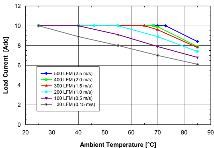
Fig. 5.0V.2: Available load current vs. ambient air temperature and airflow rates for ASQ24T10050 converter with B height pins mounted horizontally with V_{in} = 24V , air flowing from pin 3 to pin 1 and maximum FET temperature \leq 120^{\circ}C .
