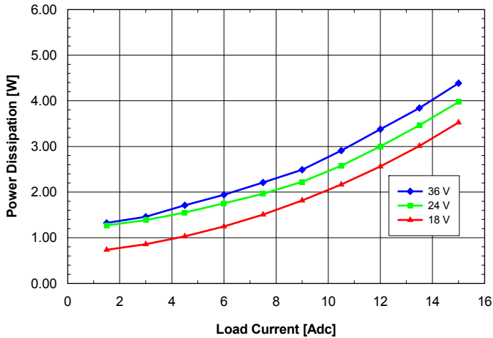
Fig. 1.0V.7: Power dissipation vs. load current and input voltage for ASQ24T/S15010 converter mounted vertically with air flowing from pin 3 to pin 1 at a rate of 300 LFM (1.5 m/s) and T_a = 25^\circ\text{C} .
