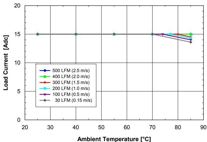
Fig. 1.8V.3: Available load current vs. ambient temperature and airflow rates for ASQ24S15018 converter mounted vertically with V_{in} = 24V , air flowing from pin 3 to pin 1 and maximum FET temperature \leq 120^{\circ}C .
