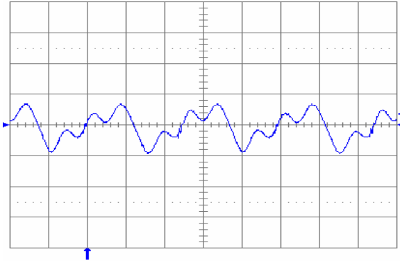
Fig. 2.0V.13: Output voltage ripple (20 mV/div.) at full rated load current into a resistive load with C_o = 10 \mu\text{F} tantalum + 1\mu\text{F} ceramic and V_{in} = 24\text{V} . Time scale: 1 \mu\text{s}/\text{div} .
